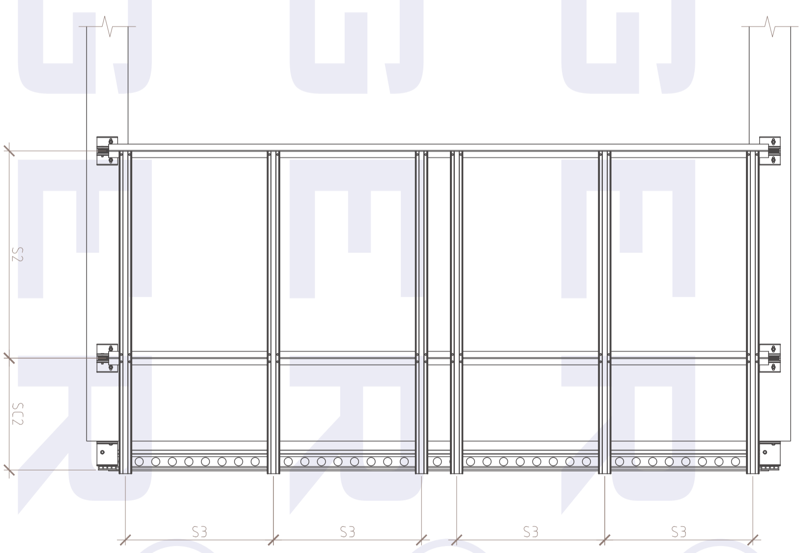
ELEVATION VIEW
